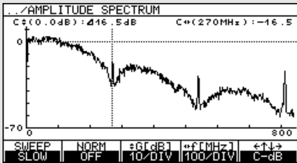
Display of amplitude spectrum up to approx. 8 MHz
