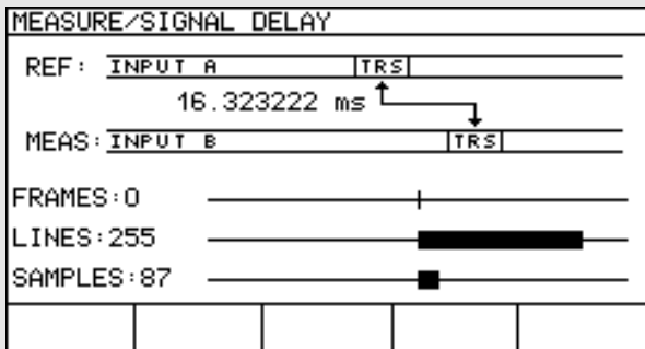
Measurement of delay between two signals over ±8 frames
