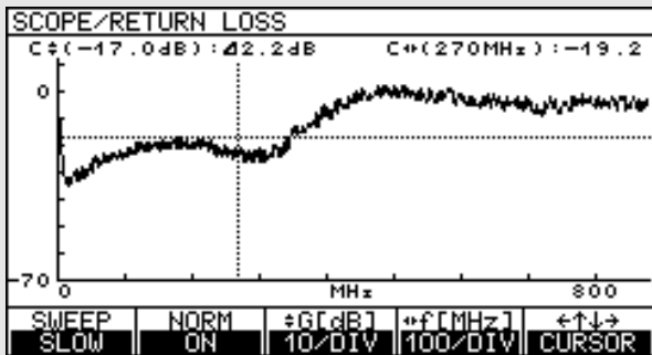
Frequency-dependent measurement of return loss using external SWR bridge
